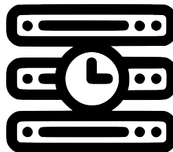
Time-sharing
